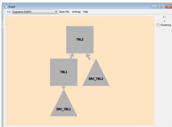
Figure 3: Projects Graph
