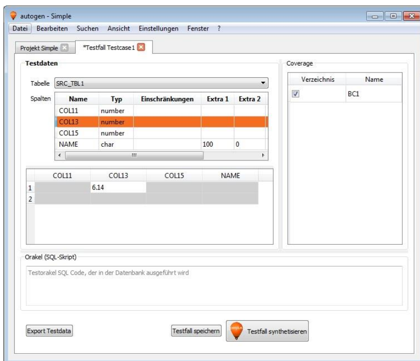
Figure 2: Testcase workspace
